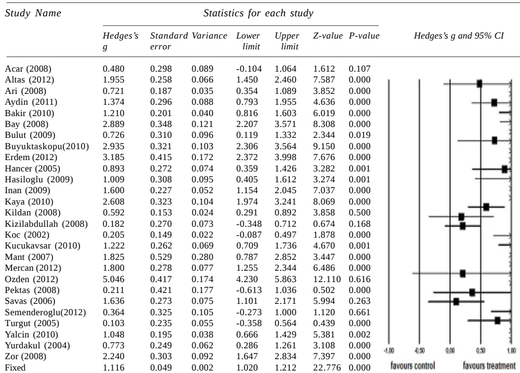
Fig. 1. Meta-analysis diagram showing the effect direction of the studies (Forest Plot)
